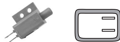
Order No. 31 - 9658 Plunger Interlock switch replaces Exmark 1-513152. Single pole, normally closed.
