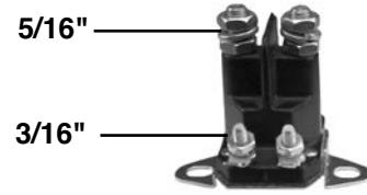
Order No. 31 - 8943 Universal Solenoid. Replaces Exmark 1-513075.
