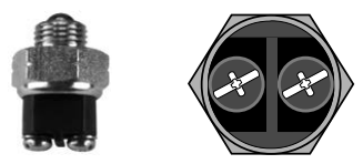
Order No. 31 - 8911 Safety switch replaces Scag 48021. Fits walkbehind mowers for "G" series PTO & "G" series PRO. 2 terminal, 9/16" mounting stem, normally open contact.
