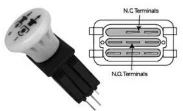
Order No. 31 - 13248 PTO switch replaces Scag 483957. 10 amp PTO switch.
