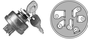
Order No. 31 - 11822 Ignition switch replaces Exmark 103-0206. 3 position, 6 terminals.
