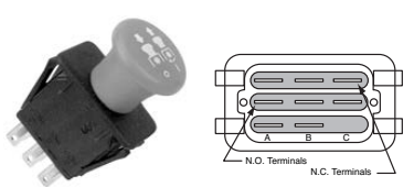
Order No. 31 - 9656 PTO switch replaces Scag 481687, 27328. Push-pull/Snap in mount. Corner terminal blank. Red Knob.
