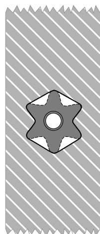
New Blade Center Hole with MTD's 6 Point Star Spindle
