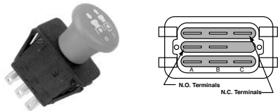
Order No. 31 - 9657 PTO switch replaces Exmark 1-633673. Middle terminal blank. Push-pull/Snap in mount. Red Knob.
