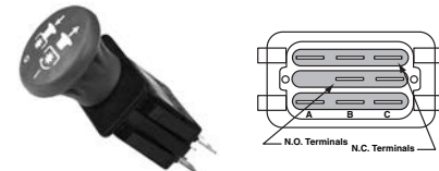
Order No. 31 - 12624 PTO switch replaces Exmark 116-0124. Electrical rating 10A@12-14VDC. Number life at rated load: 100,000 cycles resistive. (High Current). Red Knob.
