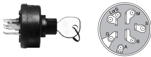
Order No. 31 - 7804 Ignition Switch replaces Scag 48798.
