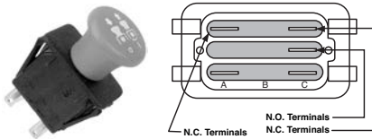
Order No. 31 - 11470 PTO switch replaces Exmark 103-5221. Fits Lazer Z, Turf Tracer, & Turf Ranger Models.Red Knob.
