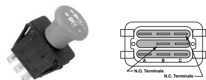
Order No. 31 - 9657 PTO switch replaces Scag 481635, 700675. Middle terminal blank. Push-pull/Snap in mount. Red Knob.
