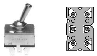
Order No. 31 - 7922 PTO switch replaces Scag 48787. Includes mounting hardware.
